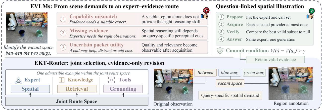
Figure 1: EKT-Router couples capability selection with evidence acquisition. Top: three conceptual failure modes of independent decisions. Bottom: the Route Space includes one expert, optional knowledge, and a budgeted tool subset, followed by acquisition, packet verification, and one answer.
