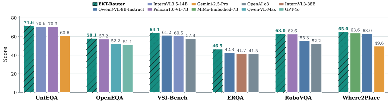
Figure 3: Embodied QA across six benchmarks (Q1) . Each panel uses its native higher-is-better metric. Results combine reported and reproduced scores under the respective evaluation protocols.
