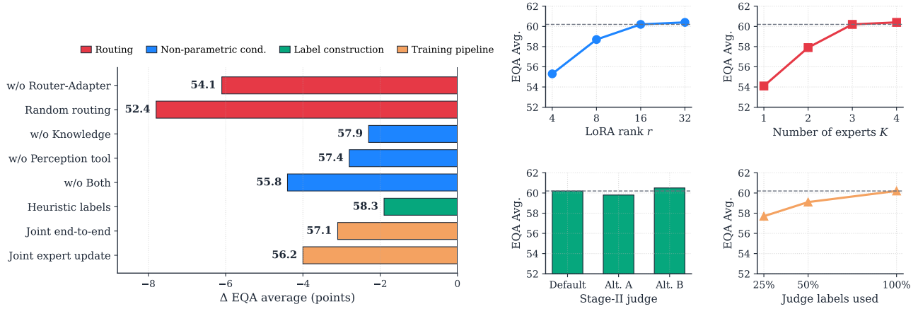
Figure 5: Ablations and sensitivity under the separate frozen protocol (Q3). Left: changes from the 60.2 full-system score. Right: LoRA rank, expert count, answer judge, and route-label coverage. Dashed lines mark the full system.
