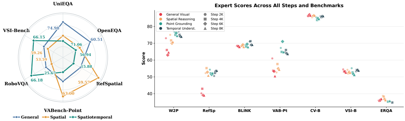
Figure 4: Expert complementarity (Q2). Left: the three deployed experts reverse rank on six representative benchmarks from the matched control. Right: candidate-checkpoint differences persist across training. Deployment retains General, Spatial Reasoning, and Spatiotemporal; the diagnostic Pointing/Grounding candidate becomes a selectable Tool action. W2P: Where2Place; RefSp: RefSpatial; VAB-Pt: VABench-Point; CV-B: CV-Bench; VSI-B: VSI-Bench.
