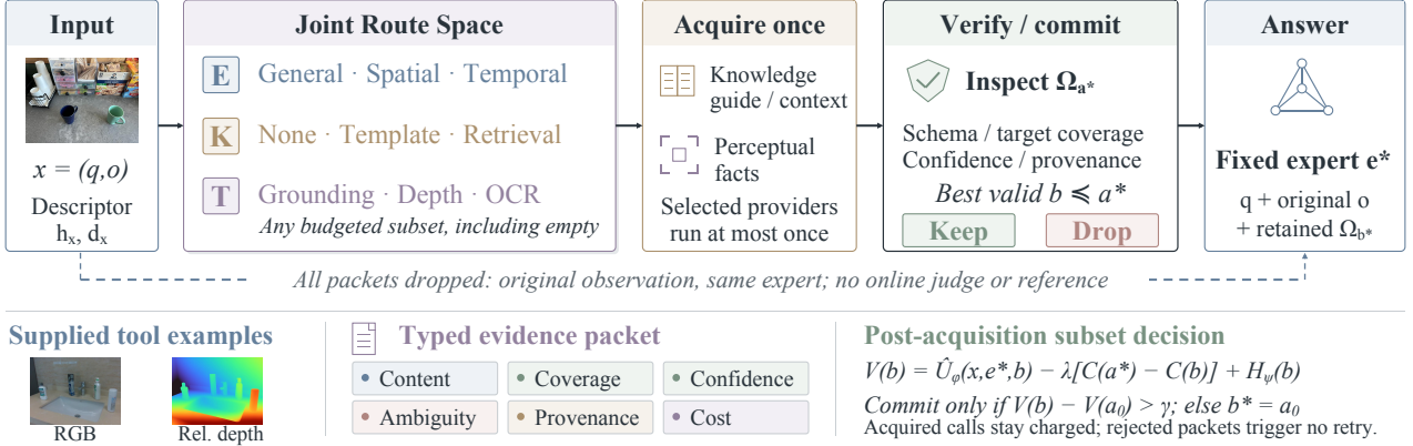
Figure 2: Overview of EKT-Router. (a) Offline : independent adaptations form the expert portfolio; evidence-free diagnostics yield capability signatures, and paired answer outcomes supervise the router and verifier. (b) Online : \phi jointly selects an expert and budgeted evidence actions. Each selected provider runs at most once. \psi scores valid packet subsets against the null reference, retaining evidence only above margin \gamma . The fixed expert answers once from the original observation and retained evidence; the dashed path preserves the evidence-free fallback.
